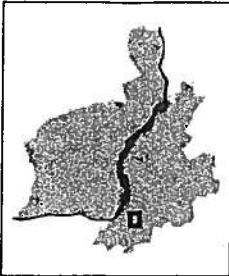
Location Reference
